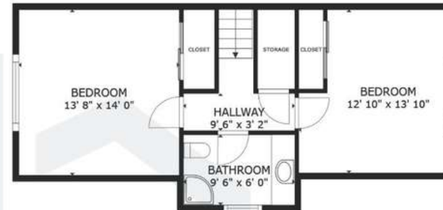
FLOOR 2
